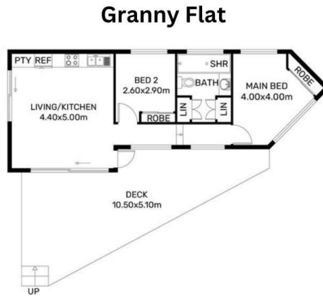
FLOOR PLAN
